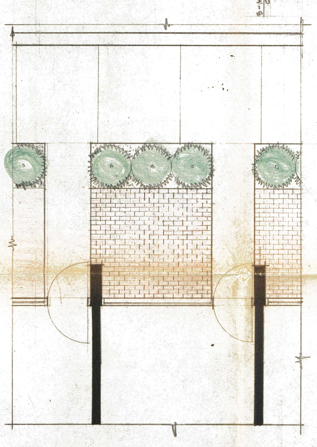
DETAIL BRICK TERRACE SCALE 1/4" = 1'-0"
